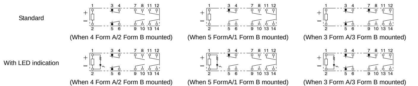
Schematic (Bottom view)
